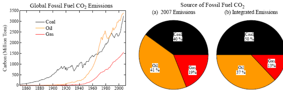
Fig. 4. Left: fossil fuel emissions versus time. Right: proportions of fossil fuel emissions in 2007 (a) and integrated emissions (b). Climate change is proportional to integrated emissions 18 .
