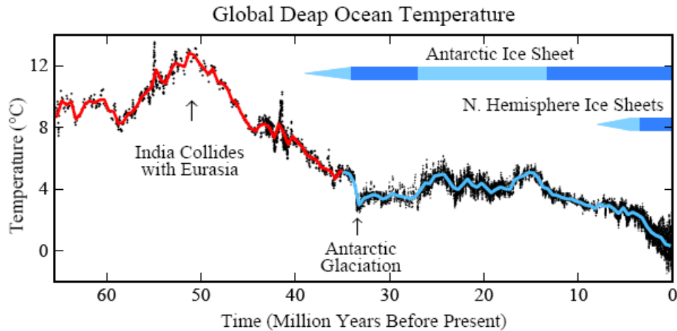
Fig. 1. Global deep ocean temperature, from Hansen et al. ( http://arxiv.org/abs/0804.1126 ). Temperature is derived from the isotopic composition of the shells of microscopic animals that lived in the deep ocean. Blue bars show the times at which ice sheets were present in each hemisphere, dark blue being the times at which the ice sheets were as large as at present or larger 2 .
