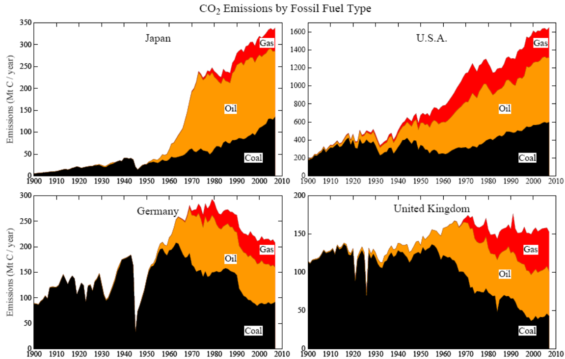
Figure 8. CO 2 emissions by fossil fuel type in four countries. Note the different scales, emissions from the United States being several times larger than those of the other countries.
