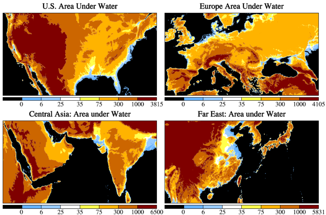
Fig. 3. Dark and light blue areas show regions that will be inundated with sea level rise of 6 and 25 meters, respectively. The last time sea level was 25 meters higher was in the Pliocene, about 3 million years ago, when the deep ocean was about 1°C warmer than today (Fig. 1); global surface temperature exceeded deep ocean temperature change in this period, but by less than a factor of two.
