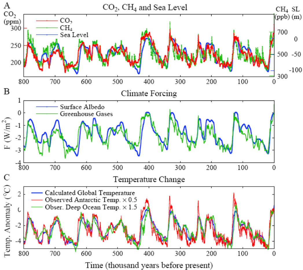
Figure 2. (A) CO 2 , CH 4 and sea level for the past 800 ky, (B) climate forcings due to changes of GHGs and ice sheet area, the latter inferred from sea level change, (C) calculated global temperature change for a climate sensitivity 3/4°C per W/m 2 compared with temperatures obtained from an Antarctic ice core and global ocean sediment cores. Polar surface temperature change is about twice global temperature change as a result of feedbacks that amplify high latitude change; deep ocean temperature change is less than the surface temperature change, because Pleistocene deep ocean temperature change is limited by the freezing point ( http://arxiv.org/abs/0804.1126 ).
